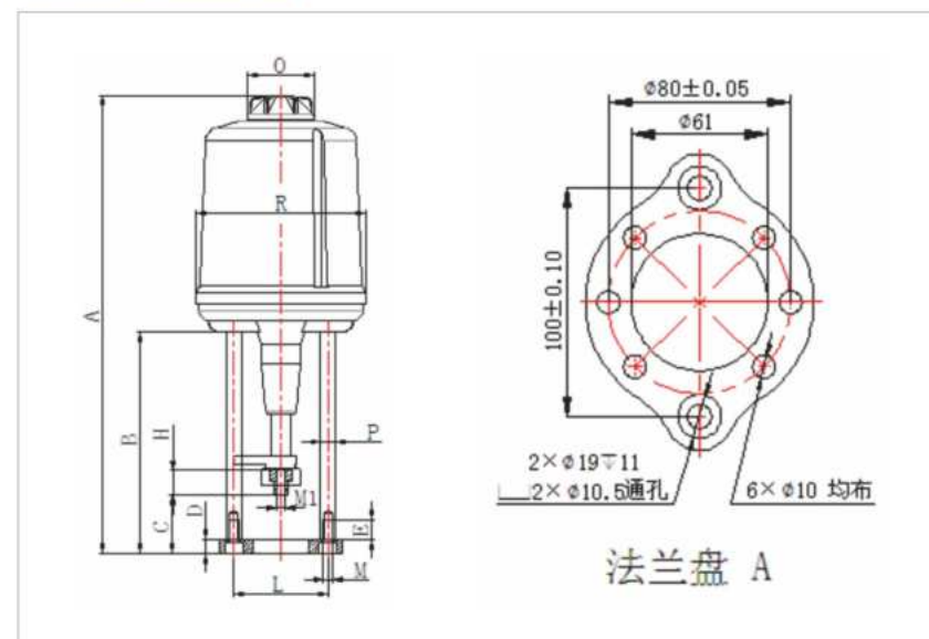
XSL100系列外形尺寸图: XSL100 Series Outline Dimensional drawing
